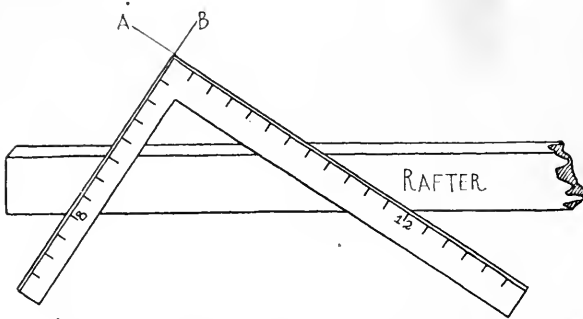
FIG. 30. SQUARE PLACED FOR PLUMB CUT.
